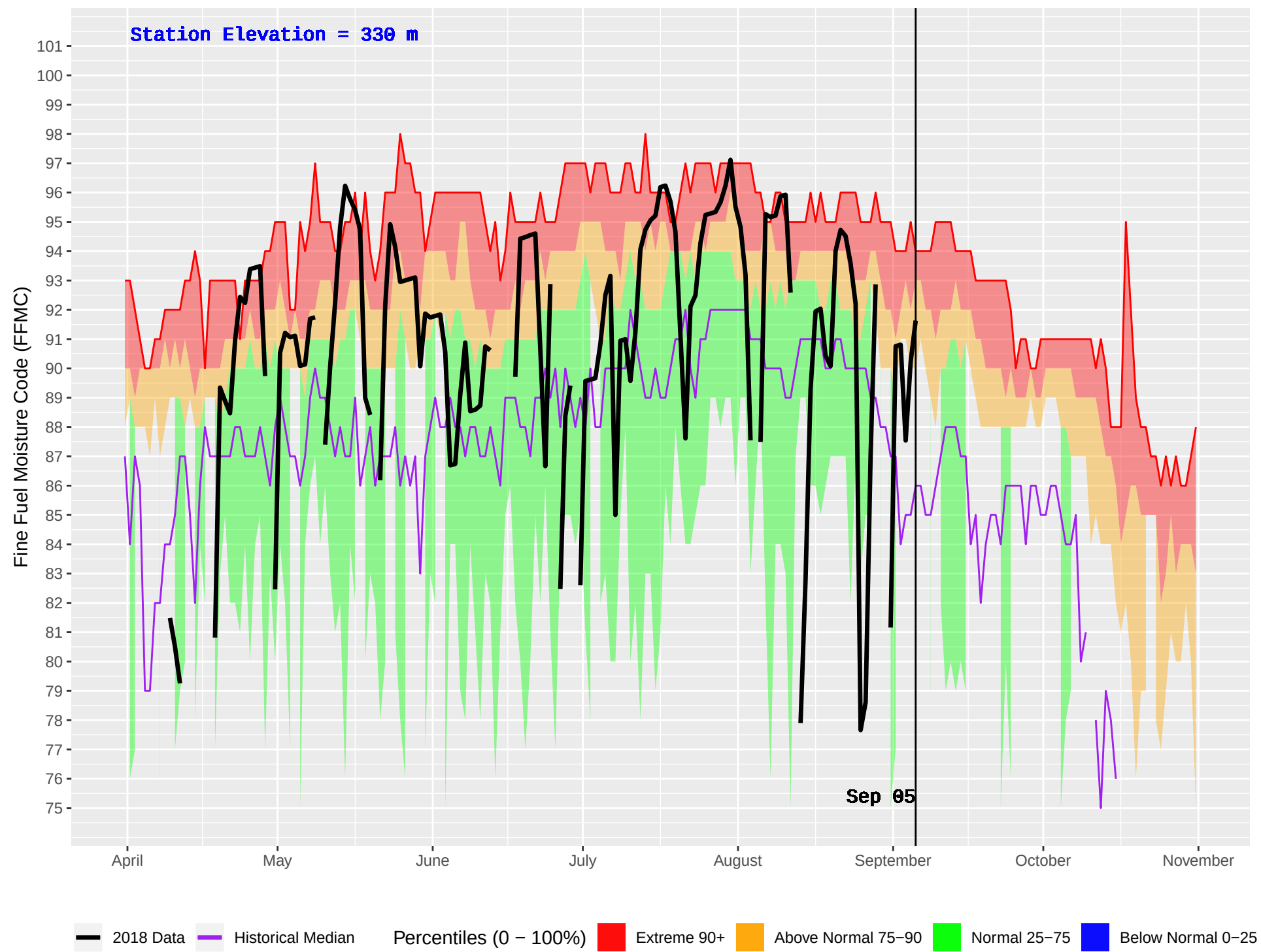
D'ARCY (292) : Historical (1978–2016) and Current (2018) Daily Fine Fuel Moisture Code (FFMC)
