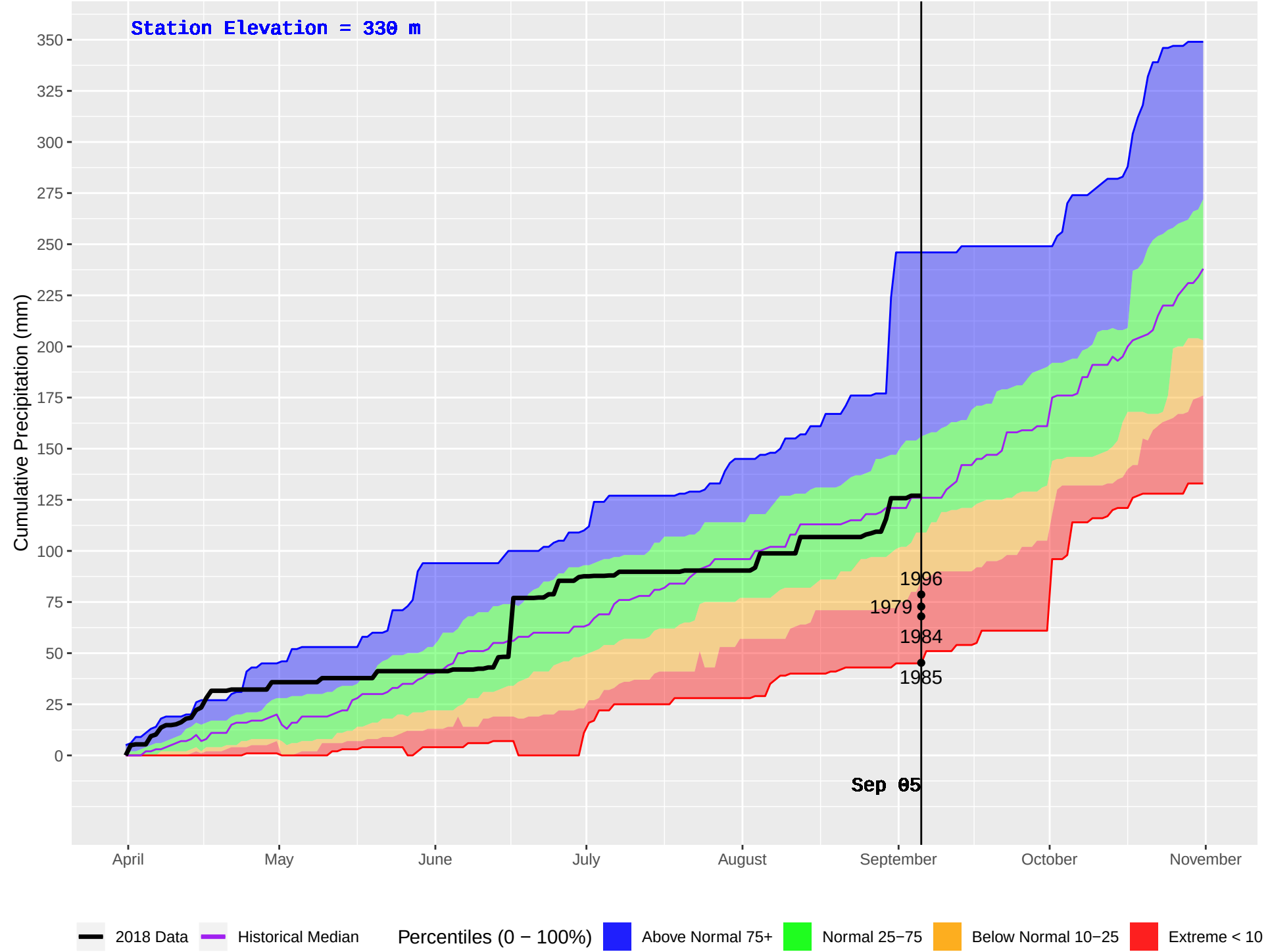
D'ARCY (292) : Historical (1978–2016) and Current (2018) Daily Cumulative Precipitation
