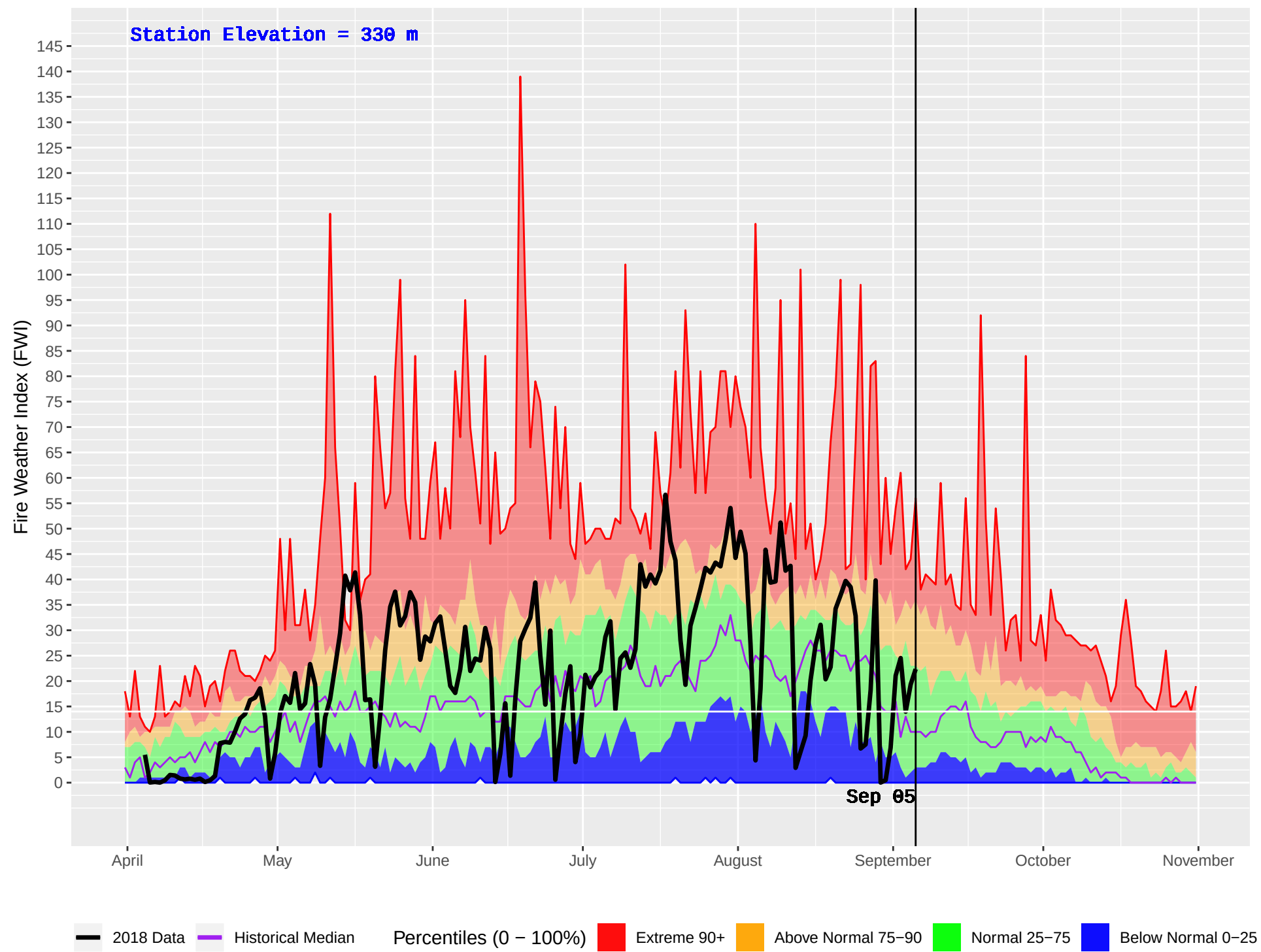
D'ARCY (292) : Historical (1978–2016) and Current (2018) Daily Fire Weather Index (FWI)
