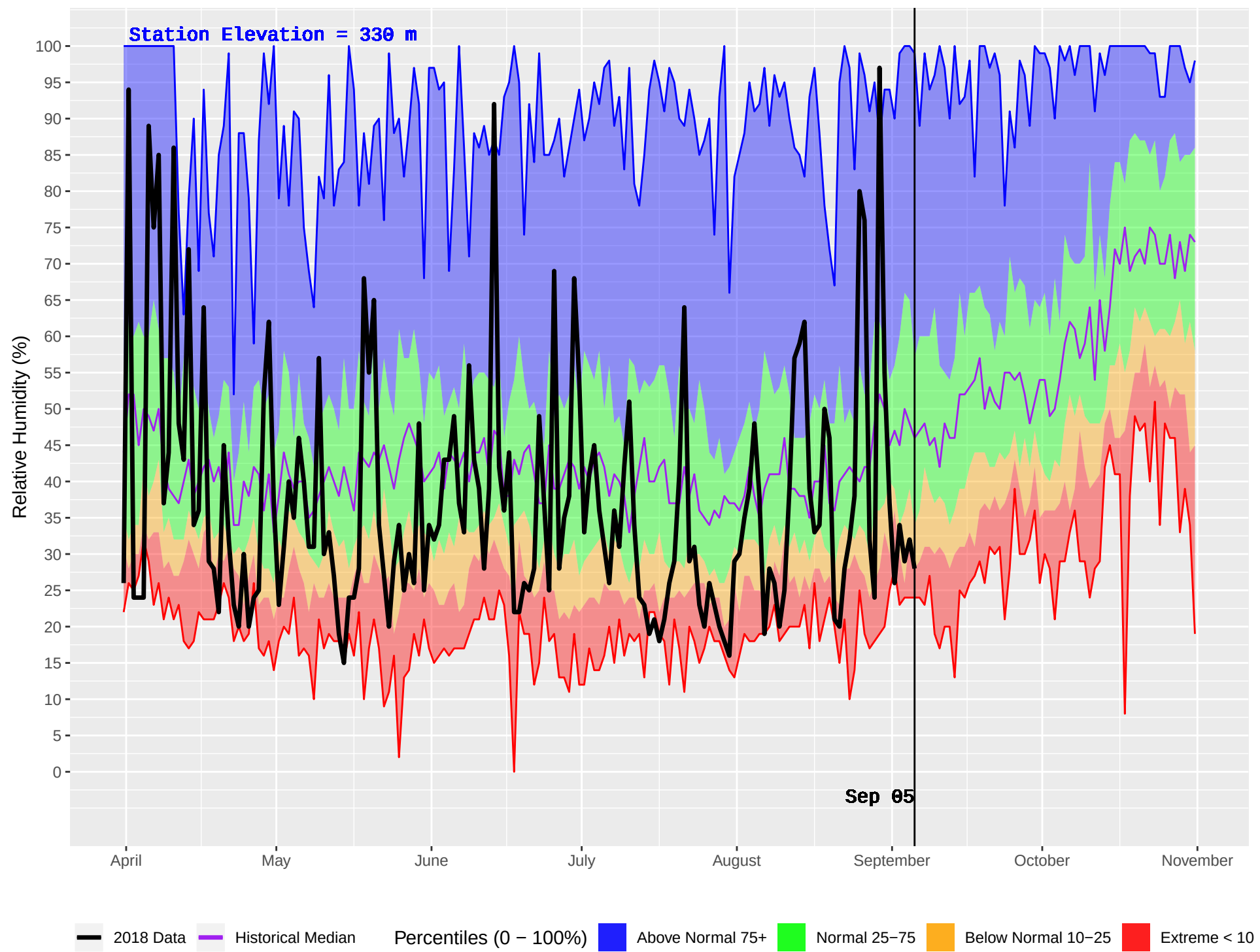
D'ARCY (292) : Historical (1978–2016) and Current (2018) Daily Relative Humidity
