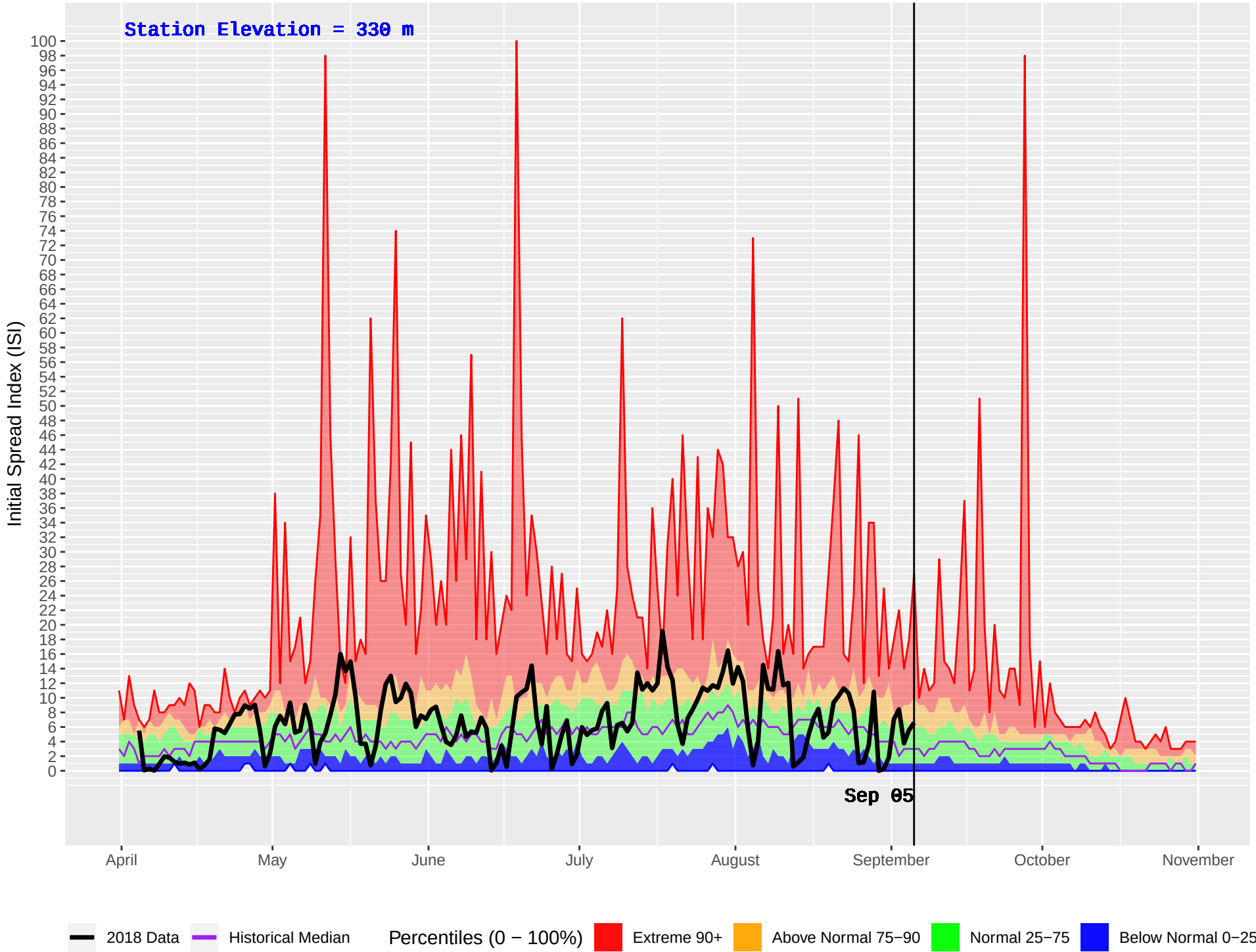
D'ARCY (292) : Historical (1978–2016) and Current (2018) Daily Initial Spread Index (ISI)
