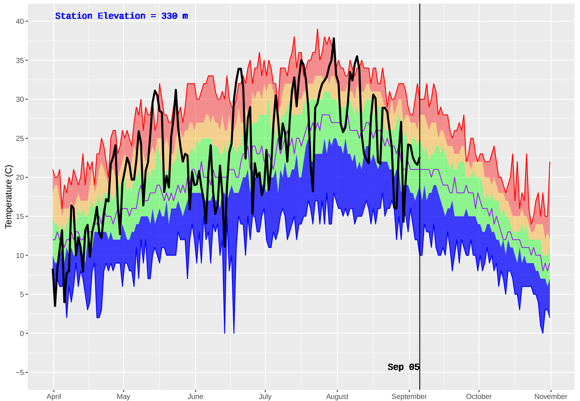
D'ARCY (292) : Historical (1978–2016) and Current (2018) Daily Temperature
